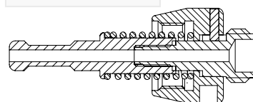
Valve head Type H Item no.: 600049
