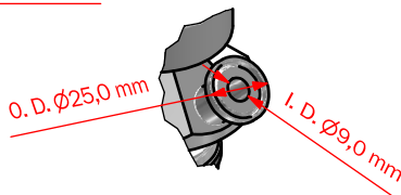
Festo Fitting QSML-M5-4
